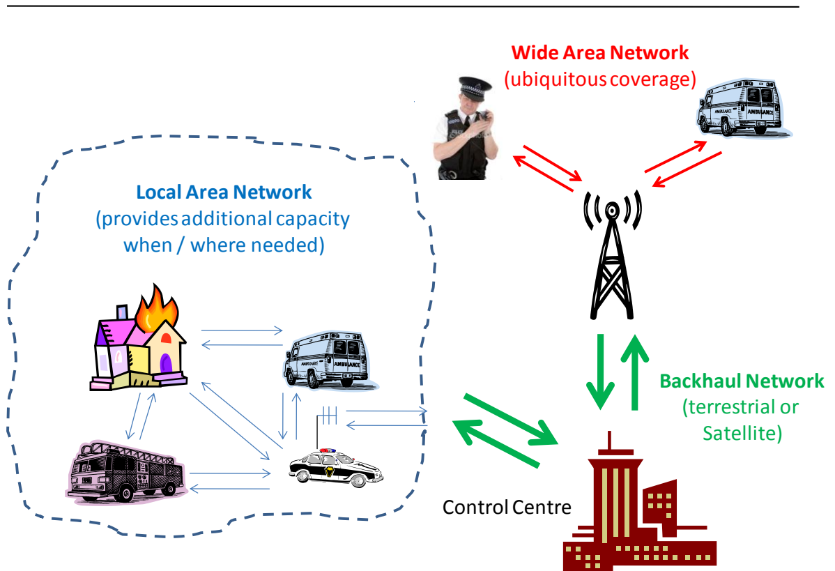
Figure 3-1: Layered Approach to Network Configuration
